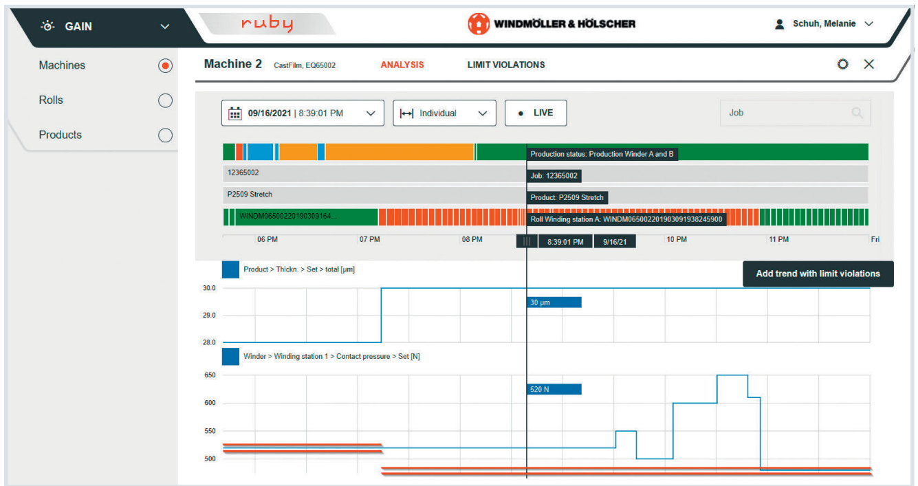
Fig. 2. The limit violation shows that the contact pressure still needs to be adjusted. © W&H
