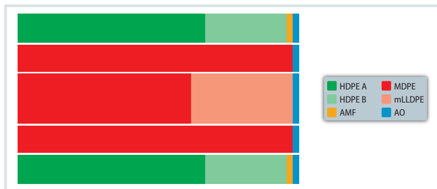
Fig. 1. Film structure of a MDO-PE 5-layer film. The height of the bar represents the thickness of the layers, the color of the bar represents the different raw materials, and the width of the bar represents the proportion of the raw material in the respective layer. Source: W&H; graphic: © Hanser
