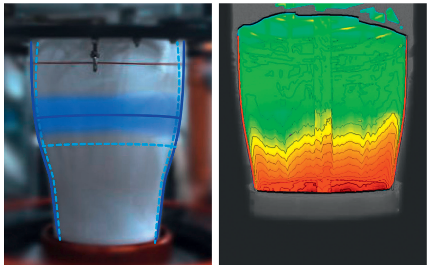
Fig. 3. Inline recording of the cooling behavior in the film bubble. The setpoints for the bubble shape and the frost line height are represented by broken lines, and the current values by continuous lines. © W&H
